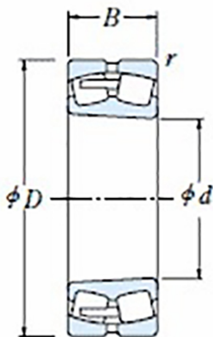
Tapered Bore
